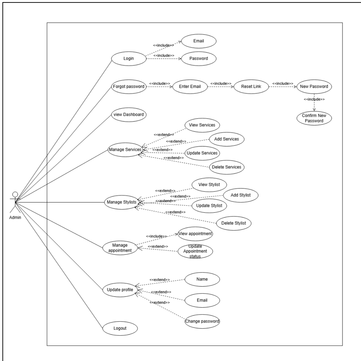
Figure 1: Admin use case diagram
