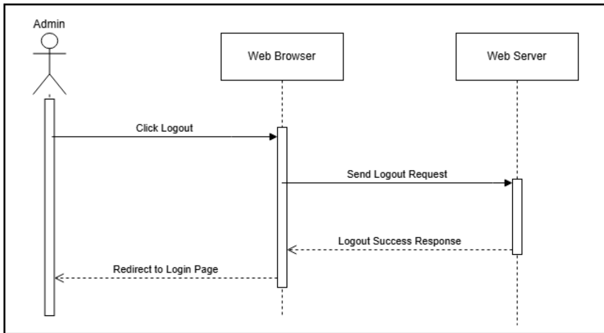
Figure 19: Admin Logout Sequence Diagram
