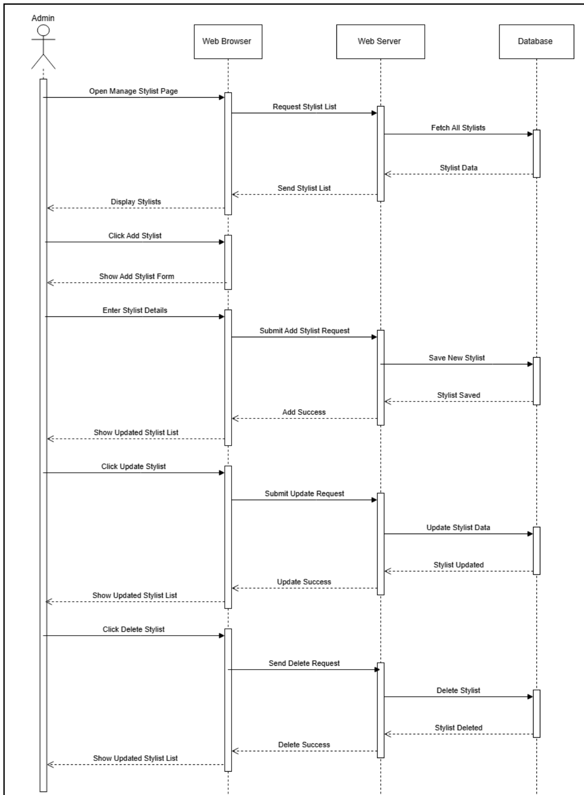
Figure 16: Manage Stylists Sequence Diagram
