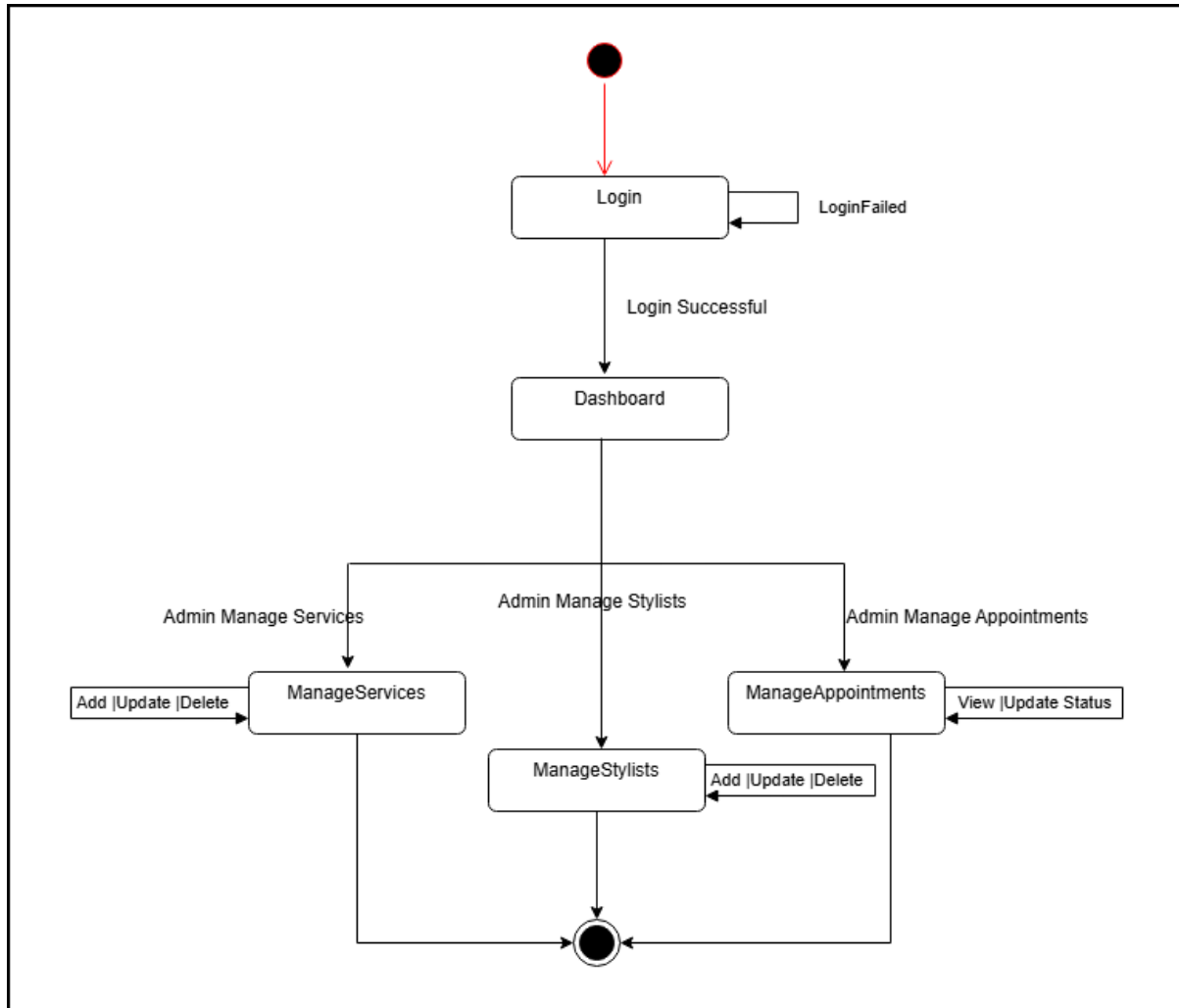
Figure 21: Admin State Diagram
