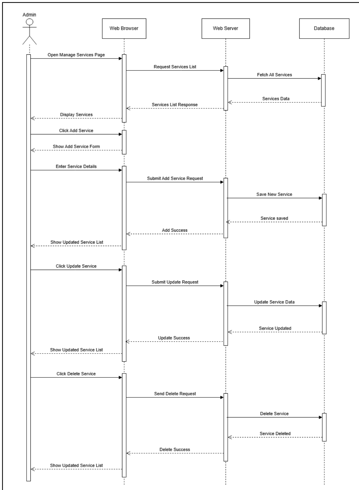
Figure 15: Manage Services Sequence Diagram
