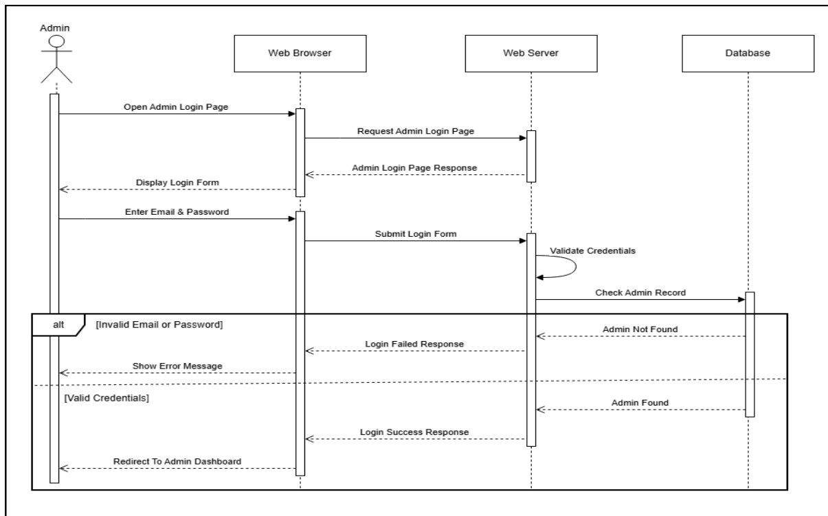
Figure 13: Admin Login Sequence Diagram
