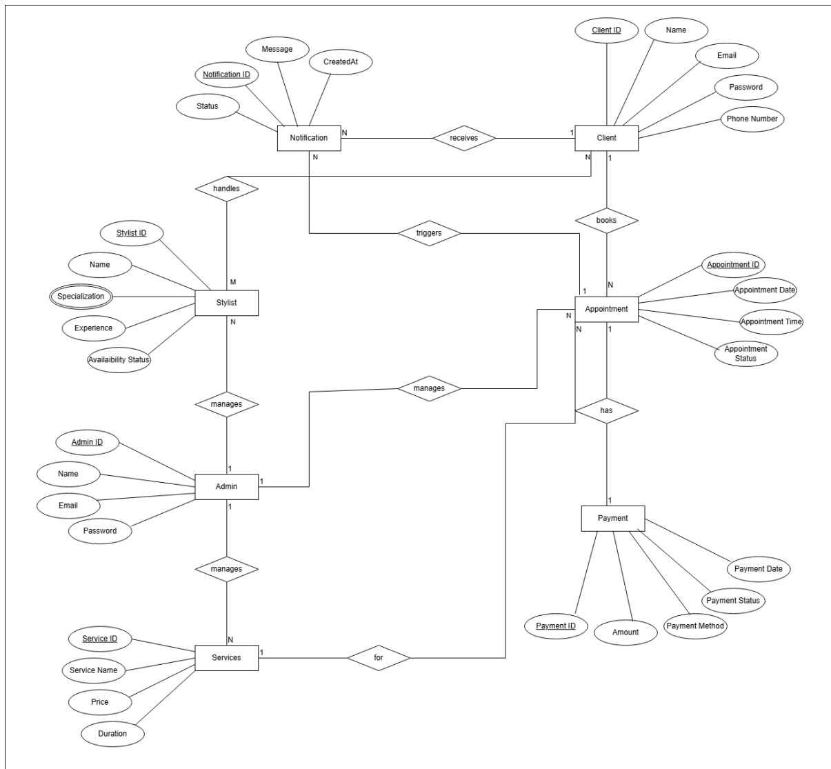
Figure 23: Entity Relationship Diagram
