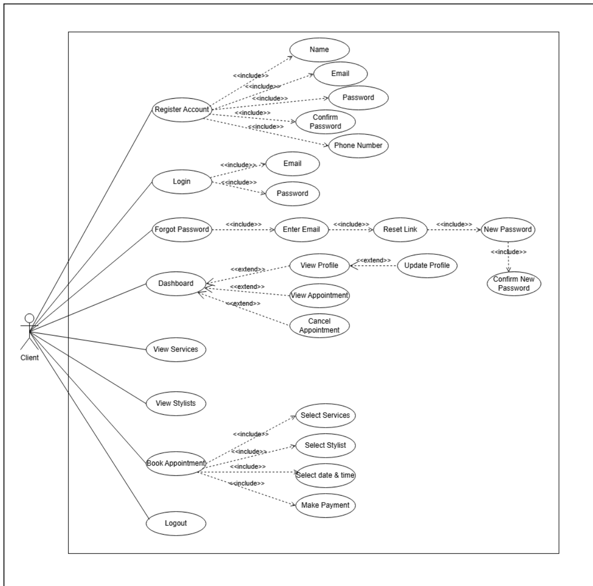
Figure 2: Client use case diagram
