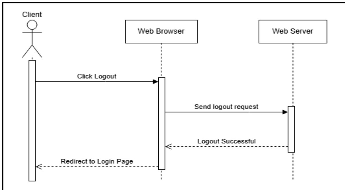
Figure 12: Client Logout Sequence Diagram
