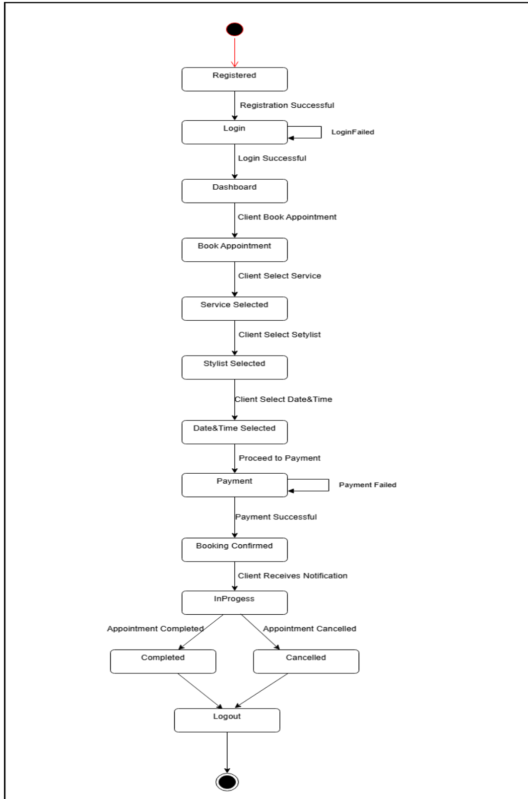
Figure 20: Client State Diagram
