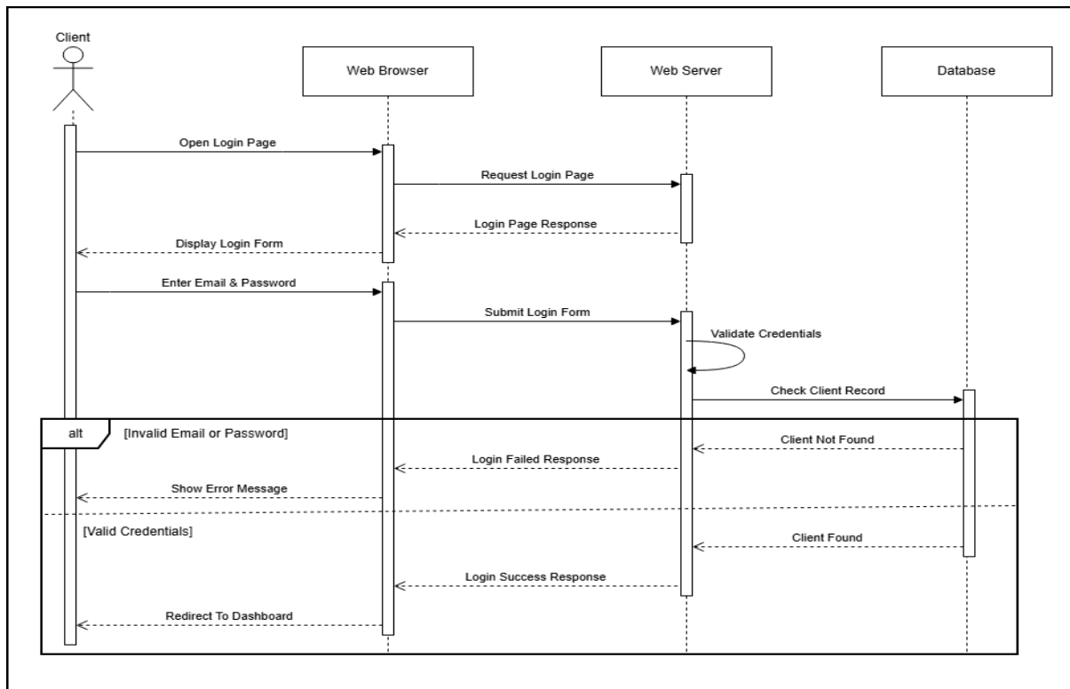
Figure 6: Client Login Sequence Diagram
