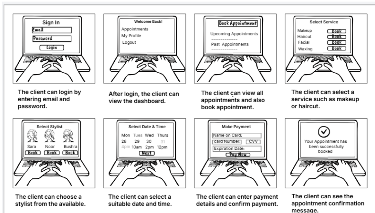
Figure 3: Storyboard for Book Appointment
