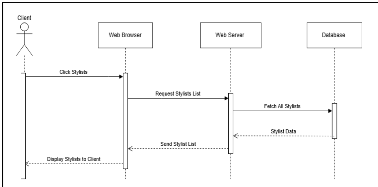
Figure 9: Client View Stylist Sequence Diagram
