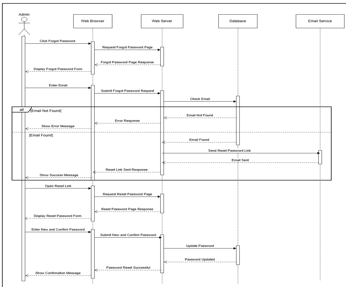
Figure 14: Admin Forgot Password Sequence Diagram
