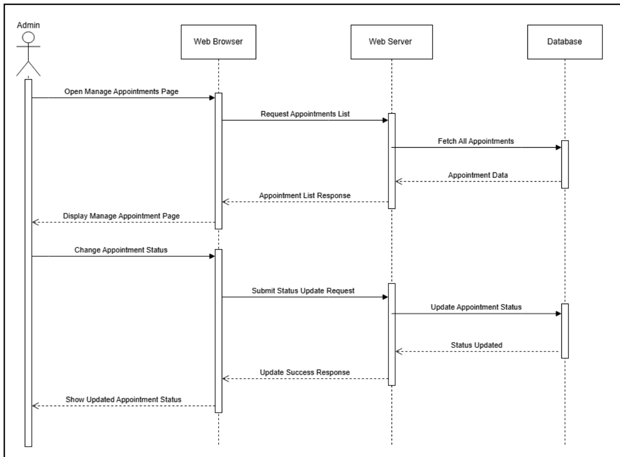
Figure 17: Manage Appointment Sequence Diagram
