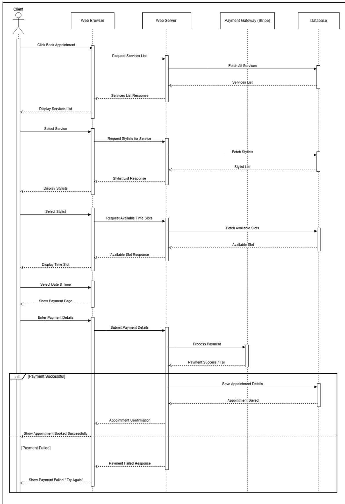
Figure 10: Book Appointment Sequence Diagram
