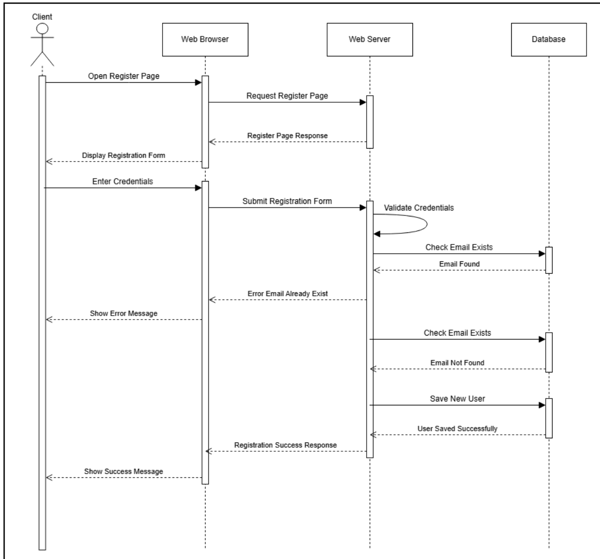
Figure 5: Client Register Sequence Diagram
