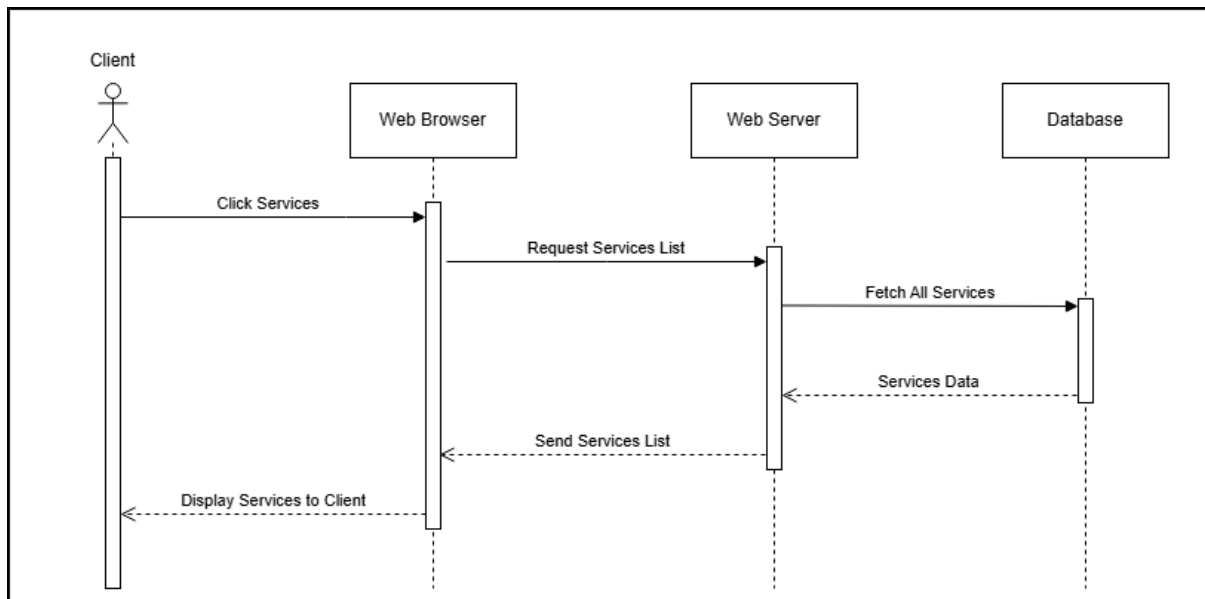
Figure 8: Client View Services Sequence Diagram
