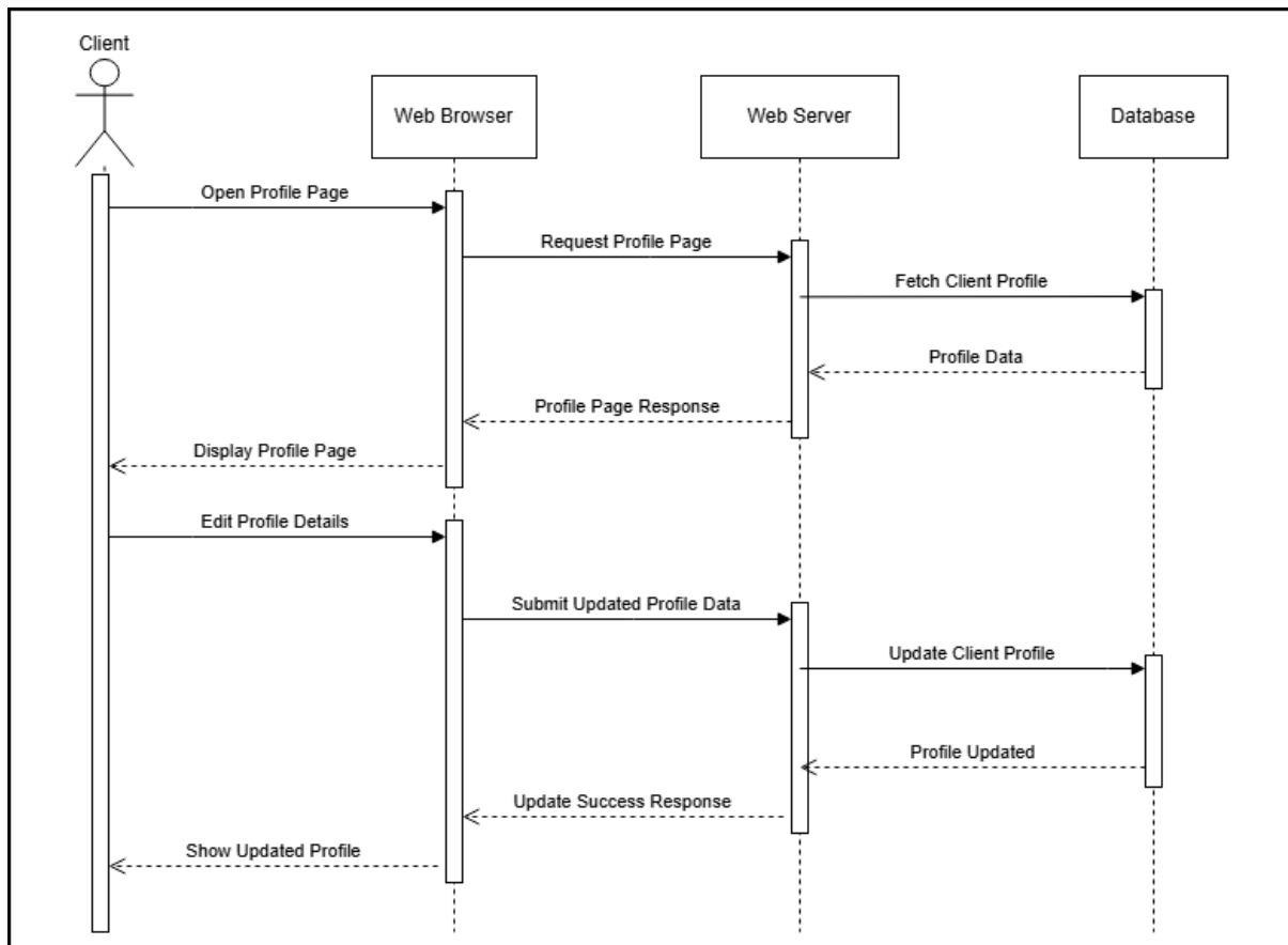
Figure 11: Client Update Profile Sequence Diagram
