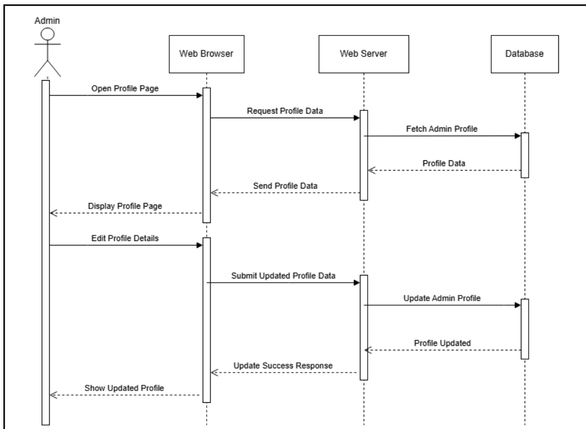
Figure 18: Admin Update Profile Sequence Diagram
